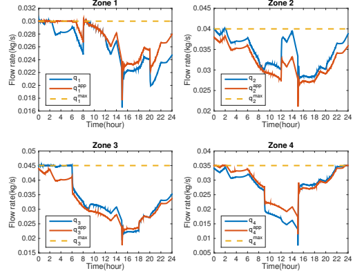
Fig. 4: Flow rates in Scenario I.
